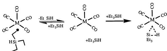
Scheme 3. Dissociative rearrangement.
