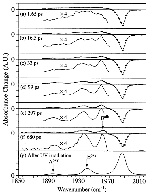
Fig. 4. Transient difference spectra in the CO stretching region for \text{Cr}(\text{CO})_6 in neat 1-hexanol at 1.65, 16.5, 33, 99, 297, 680 ps and the static difference spectra following 295 nm UV photolysis. The A and E CO stretching bands of the alkyl solvate or the OH adduct of \text{Cr}(\text{CO})_5 are labeled. These data were taken using single-element MCT detectors, described in the Section 2.
