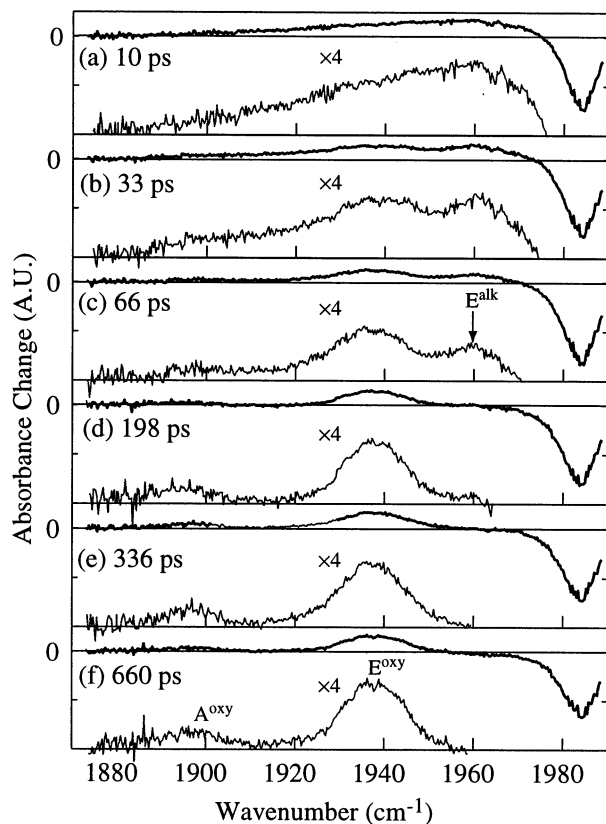
Fig. 5. Transient difference spectra in the CO stretching region for \text{Cr}(\text{CO})_6 in neat 2-propanol at 10, 33, 66, 198, 336 and 660 ps following 295 nm UV photolysis. The A and E CO stretching bands of the alkyl solvate or the OH adduct of \text{Cr}(\text{CO})_5 are labeled.
