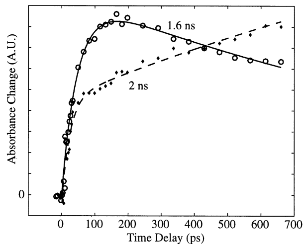
Fig. 2. Ultrafast kinetics of \text{Mo}(\text{CO})_5 in neat triethylsilane after 295 nm UV photolysis observed at: 1963 \text{ cm}^{-1} , the CO stretch of the alkyl solvate \text{Mo}(\text{CO})_5 E band (open circles); 1956 \text{ cm}^{-1} , the CO stretch of the silyl adduct \text{Mo}(\text{CO})_5 E band (closed diamonds). The time constants for the exponential fits (smooth curves) are shown in the graph.
