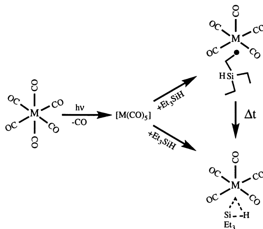
Scheme 1. Reaction sequence.
