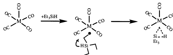
Scheme 2. Chain-walk mechanism.
