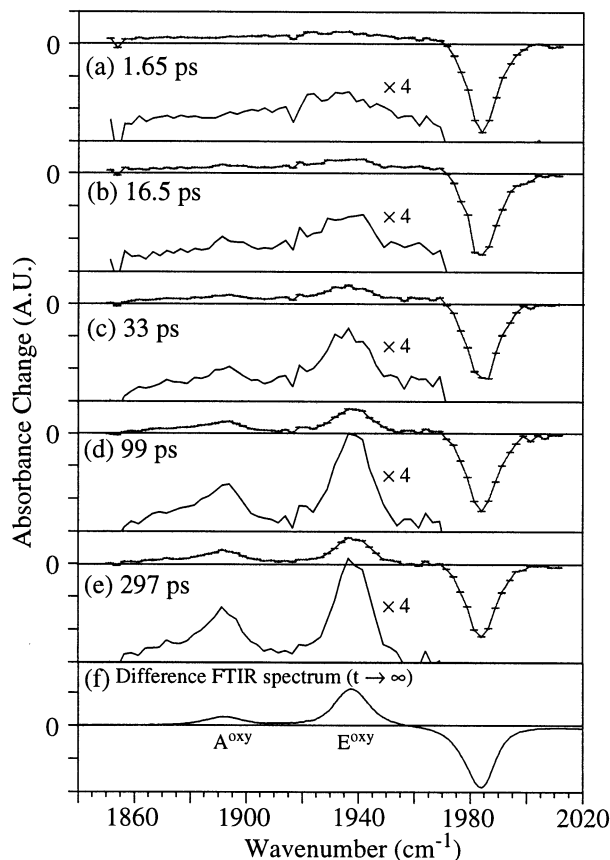
Fig. 6. Transient difference spectra in the CO stretching region for \text{Cr}(\text{CO})_6 in neat ethanol at 1.65, 16.5, 33, 99, 297 ps and the static difference spectra following 295 nm UV photolysis. The A band of the OH adduct \text{Cr}(\text{CO})_5 and E band of the alkyl solvate \text{Cr}(\text{CO})_5 are labeled. These data were taken using single-element MCT detectors, described in the Section 2.
