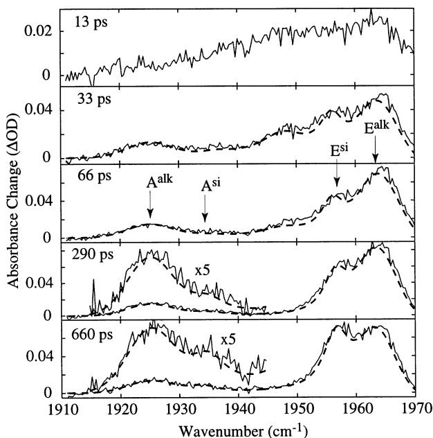
Fig. 1. Transient difference spectra in the CO stretching region for Mo(CO) 6 in neat triethylsilane at 13, 33, 66, 290 and 660 ps following 295 nm UV photolysis. The A and E CO stretching bands of the alkyl solvate or silyl adduct of Mo(CO) 5 are labeled. The fit to the data appears as a dashed line.
