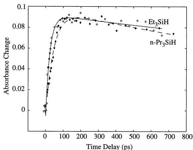
Fig. 3. Comparison of the ultrafast kinetics of the alkyl solvate \text{Cr}(\text{CO})_5 in neat triethylsilane and in neat tri- n -propylsilane after 295 nm UV photolysis observed at: the CO stretch of the alkyl solvate \text{Cr}(\text{CO})_5 E band in triethylsilane (open circles); the CO stretch of the alkyl solvate \text{Cr}(\text{CO})_5 E band in tri- n -propylsilane \text{Cr}(\text{CO})_5 (closed diamonds).
