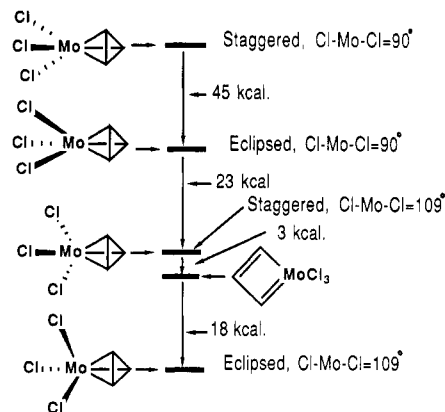
Figure 5. Ground-state energy difference of several metallatetrahedranes and the metallacyclobutadiene at the GVB (6/12) level.
