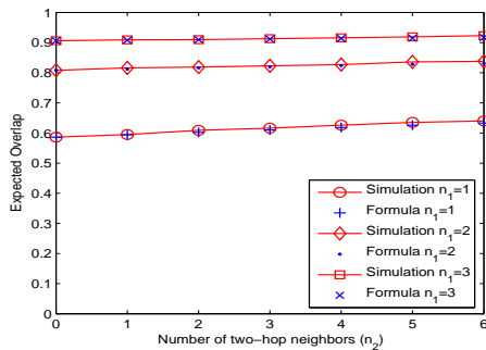
Fig. 8: Expected overlap values from simulation and formula with different n_1 and n_2 counts and when R_t/R_s=1 .
