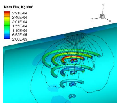
FIGURE 3: Mass flux contours in the conical dryer superimposed with the streamtraces
