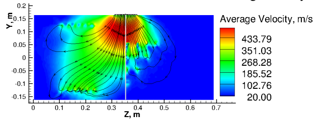
FIGURE 5: Average velocity contours for the two condenser designs
