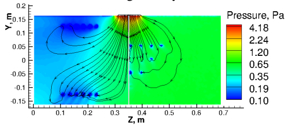
FIGURE 4: Pressure contours in the YZ plane for the two condenser designs in the YZ plane
