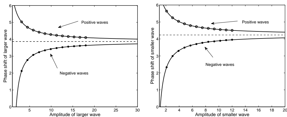
FIGURE 4. Overtaking collisions of a large and a small solitary wave with a constant amplitude ratio of 3 : 2. The left panel shows the magnitude of the phase shift of the larger waves |\theta_L| , and the right panel shows the magnitude of the phase shift of the smaller waves |\theta_S| . The circles denote the interaction of two positive waves, and the dots denote the interaction of two negative waves. The solid curves represent a rational curve fit, and the dashed line is the horizontal asymptote of both curve fits.
