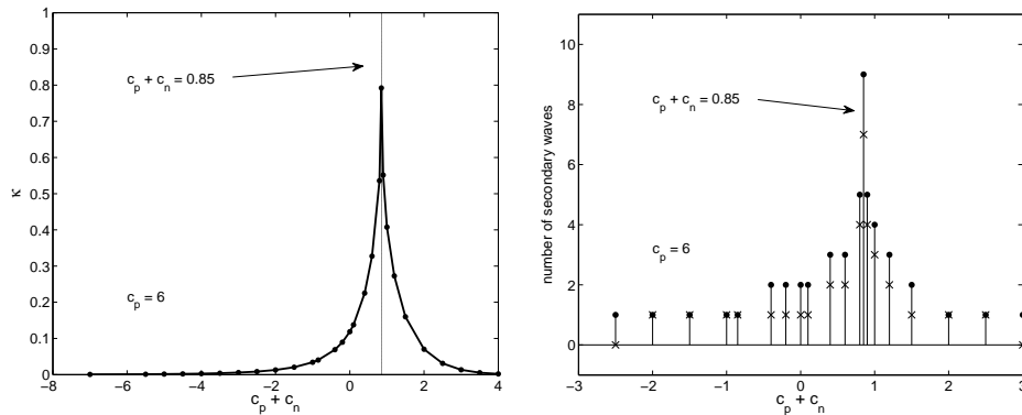
FIGURE 7. The left panel displays the inelasticity \kappa of the head-on collision of a positive and a negative solitary wave as a function of c_p + c_n . The positive solitary wave is kept constant at the speed c_p = 6 , and the velocity of the negative solitary wave is varied. The largest value of \kappa appears precisely at c_p + c_n = 0.85 . The right panel shows data from the same experiments, and records the number of secondary positive and negative solitary waves created after the collision. The number of positive secondary waves is graphed with dots, and the number of negative waves is graphed with an \times .
