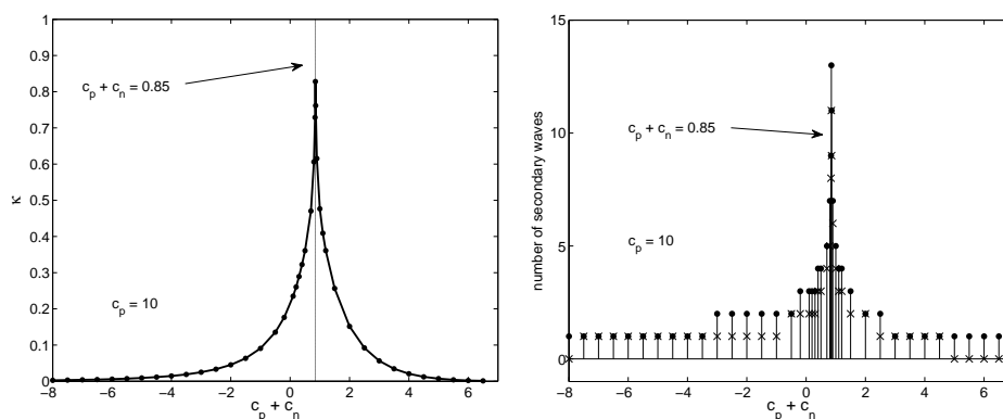
FIGURE 8. The left panel displays the inelasticity \kappa of the head-on collision of a positive and a negative solitary wave as a function of c_p + c_n . The positive solitary wave is kept constant at the speed c_p = 10 , and the velocity of the negative solitary wave is varied. The largest value of \kappa appears precisely at c_p + c_n = 0.85 . The right panel shows data from the same experiments, and records the number of secondary positive and negative solitary waves created after the collision. The number of positive secondary waves is graphed with dots, and the number of negative waves is graphed with an \times .
