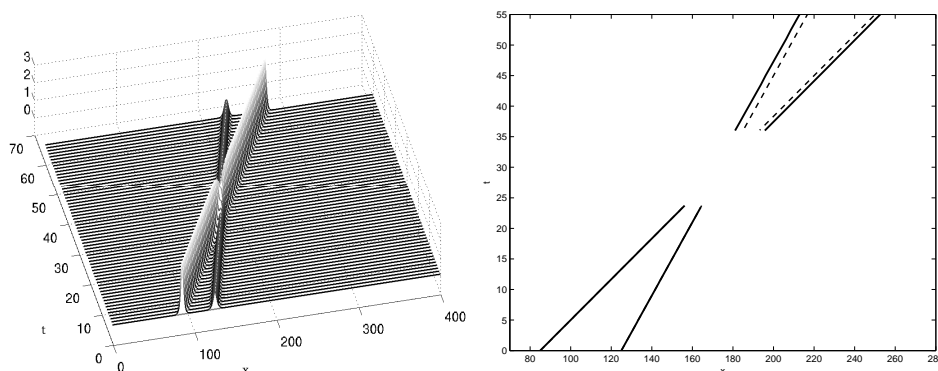
FIGURE 1. Interaction of two positive solitary waves in equation (1.1). The left panel shows the time evolution of the spatial profile. The scale is such that the dispersive tail due to the inelasticity cannot be seen. The right panel shows the positions of the maxima of the two waves as functions of t . The solid line shows the actual position of the maxima, while the dashed line indicates the position of the maxima in the case that no collision has taken place.
