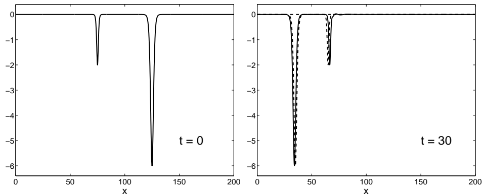
FIGURE 3. Interaction of two negative solitary waves. In the right panel, the phase shift and the production of dispersive oscillations behind the smaller solitary wave is clearly visible.
