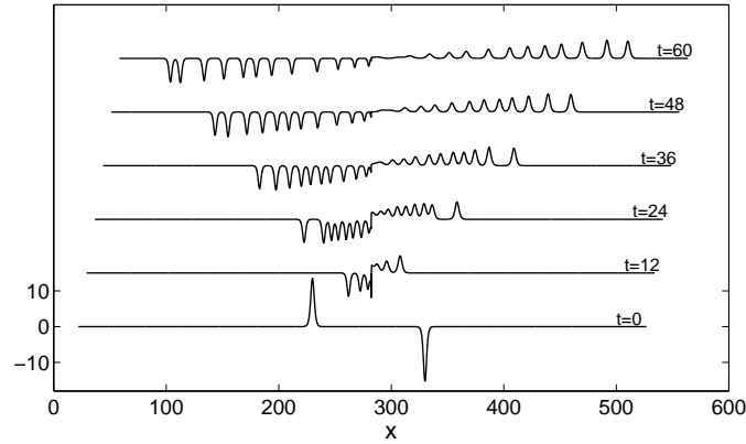
FIGURE 6. Interaction of a positive and a negative solitary wave at resonance. The wave speed of the positive solitary wave is c = 10 . The wave speed of the negative solitary wave is c = -9.15 . The figure shows snapshots of the solutions at different times, as indicated at the right end of the respective curve. A violent, nearly singular interaction can be seen, and the formation of secondary solitary waves is observed as the main waves pull from the interaction region.
