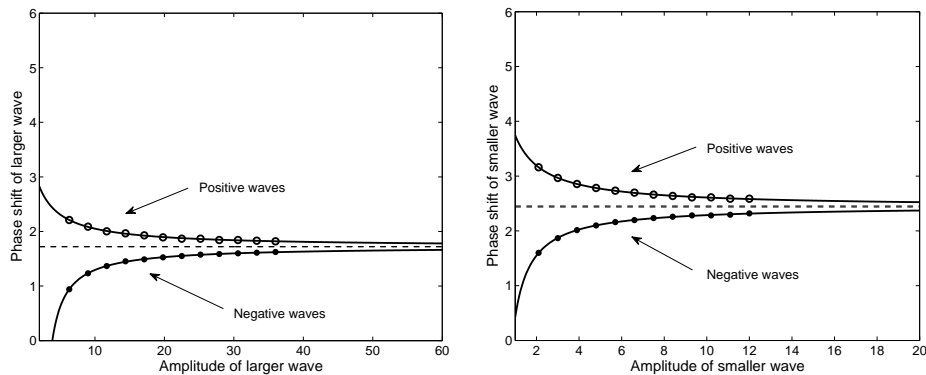
FIGURE 5. Overtaking collisions of a large and a small solitary wave with a constant amplitude ratio of 3 : 1. The left panel shows the magnitude of the phase shift of the larger waves |\theta_L| , and the right panel shows the magnitude of the phase shift of the smaller waves |\theta_S| . The circles denote the interaction of two positive waves, and the dots denote the interaction of two negative waves. The solid curves represent a rational curve fit, and the dashed line is the horizontal asymptote of both curve fits.
