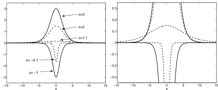
FIGURE 2. Positive and negative solitary wave profiles, for velocities c = 1.1 , c = 2 , c = 3 , and c = -0.1 , c = -1 . The right panel shows a close-up of the waves which shows the different spatial decay of positive and negative solitary waves.
