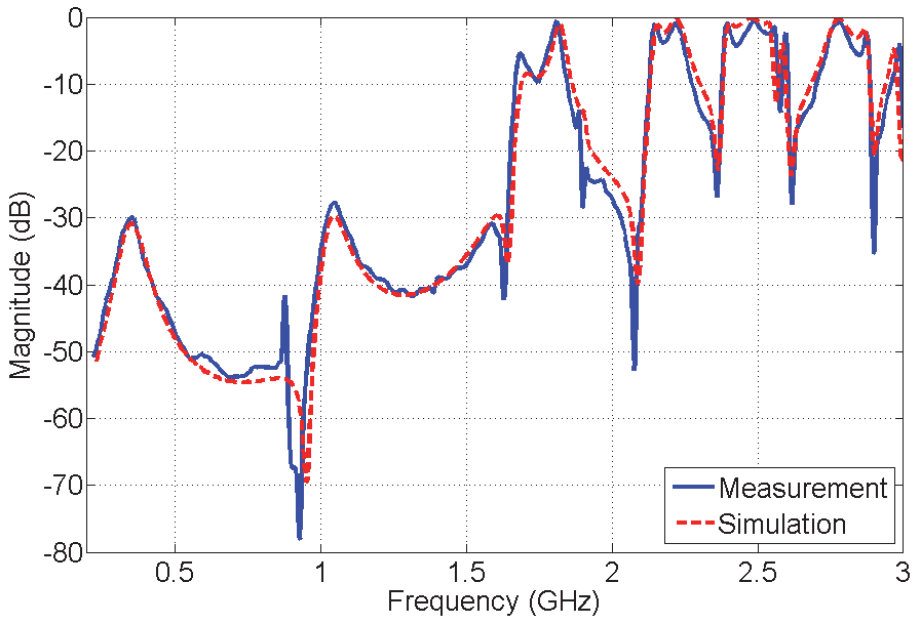
Fig. 2. Comparison between measurement and simulation.
