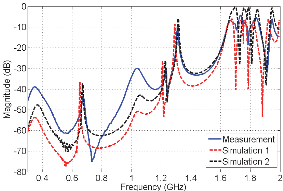
Fig. 4. Comparison between measurement and simulations.
