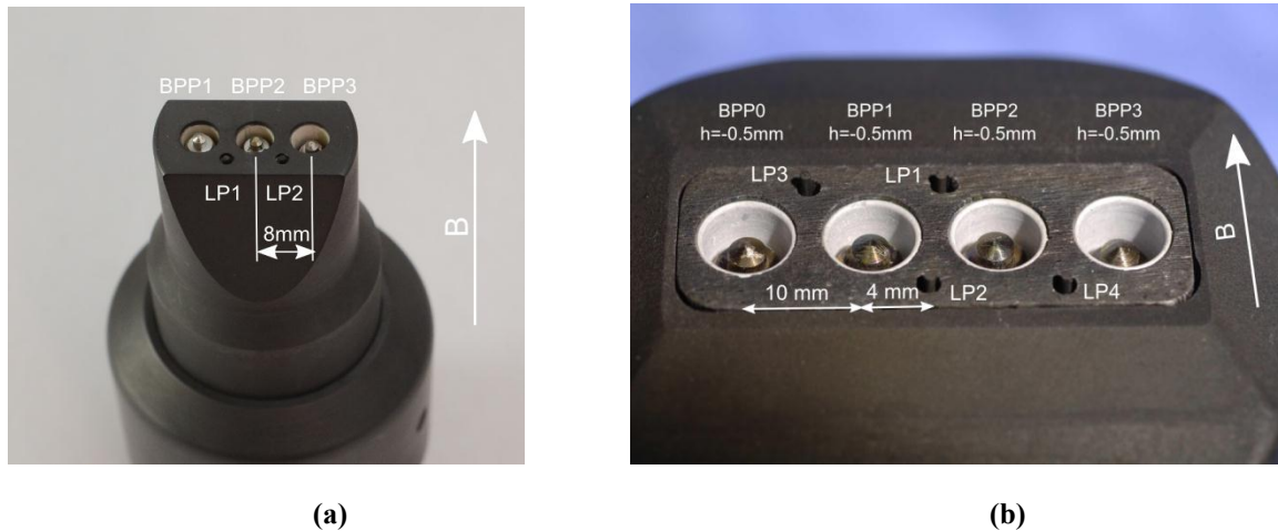
Fig. 1: (a) - Picture of the ball-pen probe (BPP) head used in COMPASS midplane manipulator. It consists of three ball-pen probes made of stainless steel collector and alumina shielding tube and two graphite Langmuir probes. The front side of the probe head has a diameter of 3 cm. (b) - Picture of the ball-pen probe head used in AUG. The probe head has four BPPs made of stainless steel collector and boron nitride shielding tube. In addition, there are four graphite Langmuir probes. The front side of the probe head has a diameter of 5 cm.
