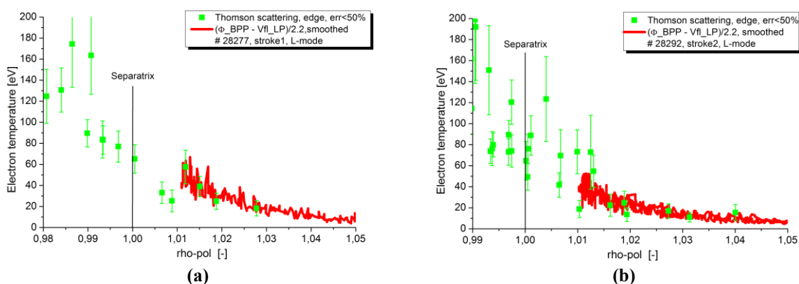
Fig. 3: Radial profiles of the electron temperature measured by BPP/LP (red line) and Thomson scattering (green squares) during L-mode discharge with NBI (a) or ECR (b) heating on ASDEX Upgrade.
