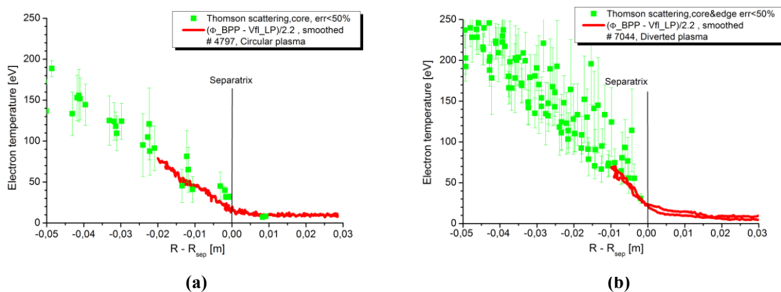
Fig. 2: Radial profiles of the electron temperature measured by BPP/LP (red line) and Thomson scattering (green squares) during circular (a) and diverted (b) plasma on tokamak COMPASS.
