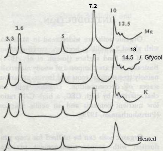
Fig. 1. X-ray diffractograms of the clay fraction from PI (0-15 cm).
