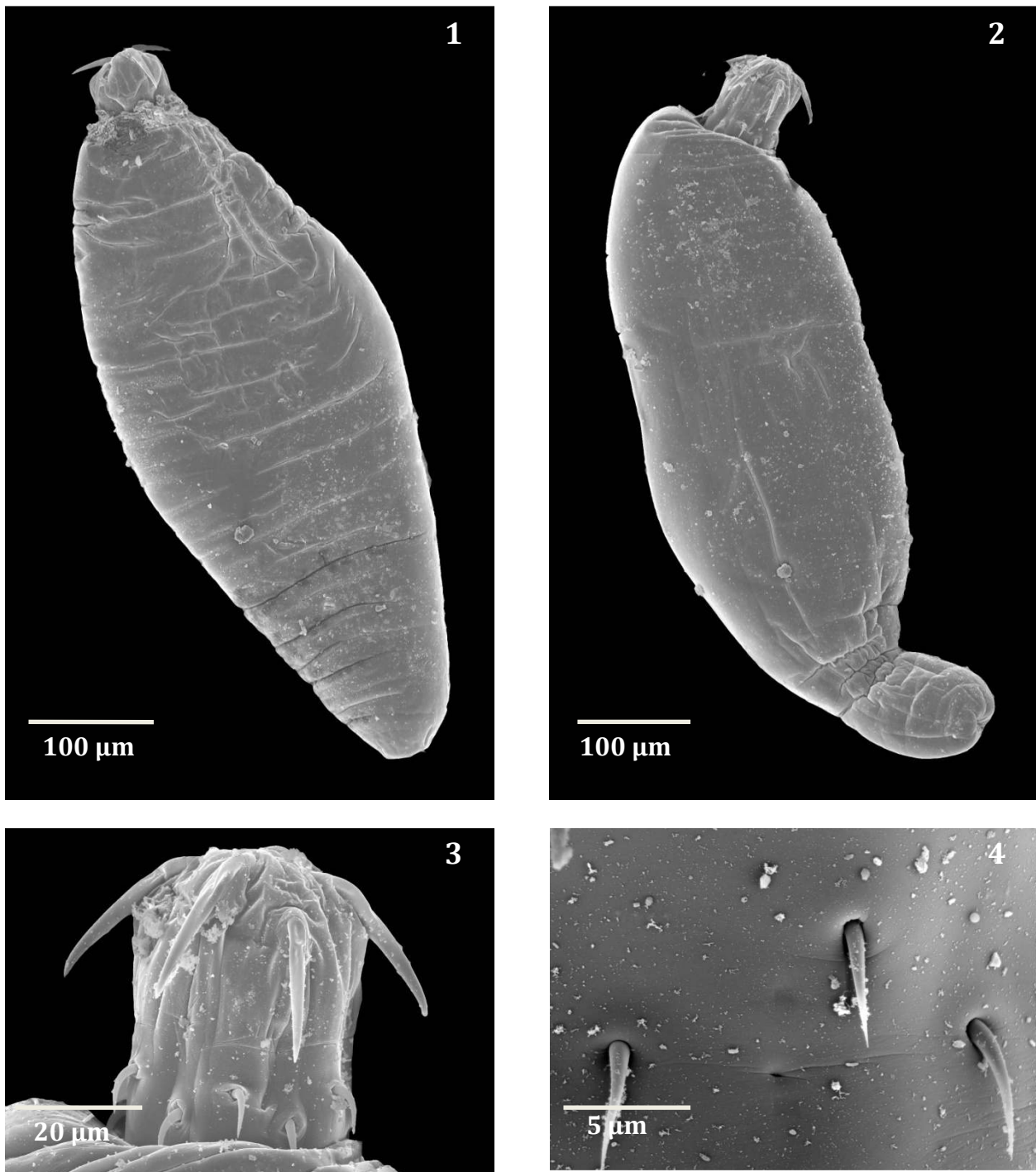
Figures 1-4. SEM of Acanthogyrus (Acanthosentis) tilapiae from Lake Malawi cichlids. 1. A male worm. 2. A female worm. 3. The proboscis of a male worm showing the alternate placement of hooks in the anterior ring. 4. Posterior hooks and a sensory pit (lower center) of another proboscis.
