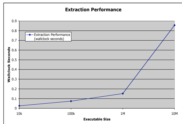
Figure 4: The extraction of the correct binary image from the fat-binary file was found to dominate the gridrun execution time. In order to test the extraction performance, artificial binary files of various sizes were constructed using a randomly generated data. The test platform in this case was a Mac G4 notebook computer (the slowest platform).
