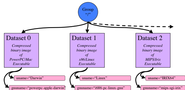
Figure 1: Schematic of the GridRun fat-binary file format.
