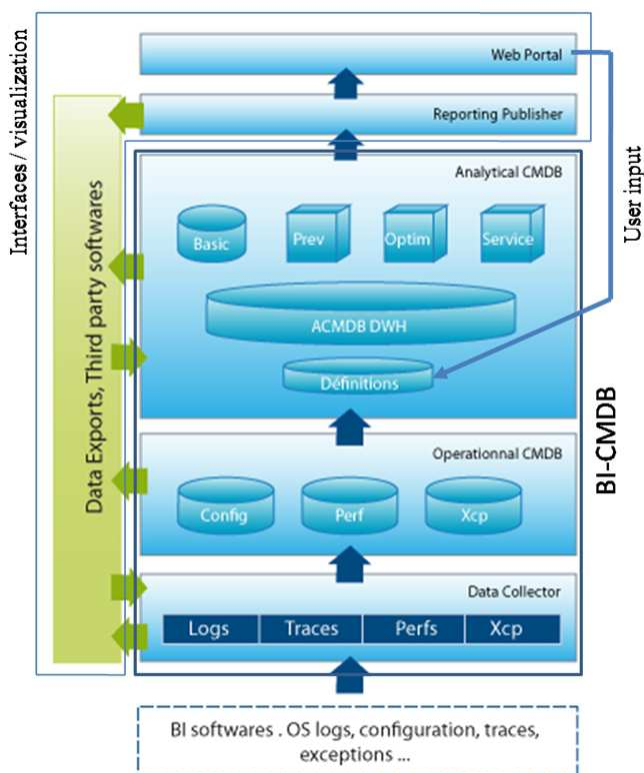
Fig. 1. The SP2 BI-CMDB simplified schema
