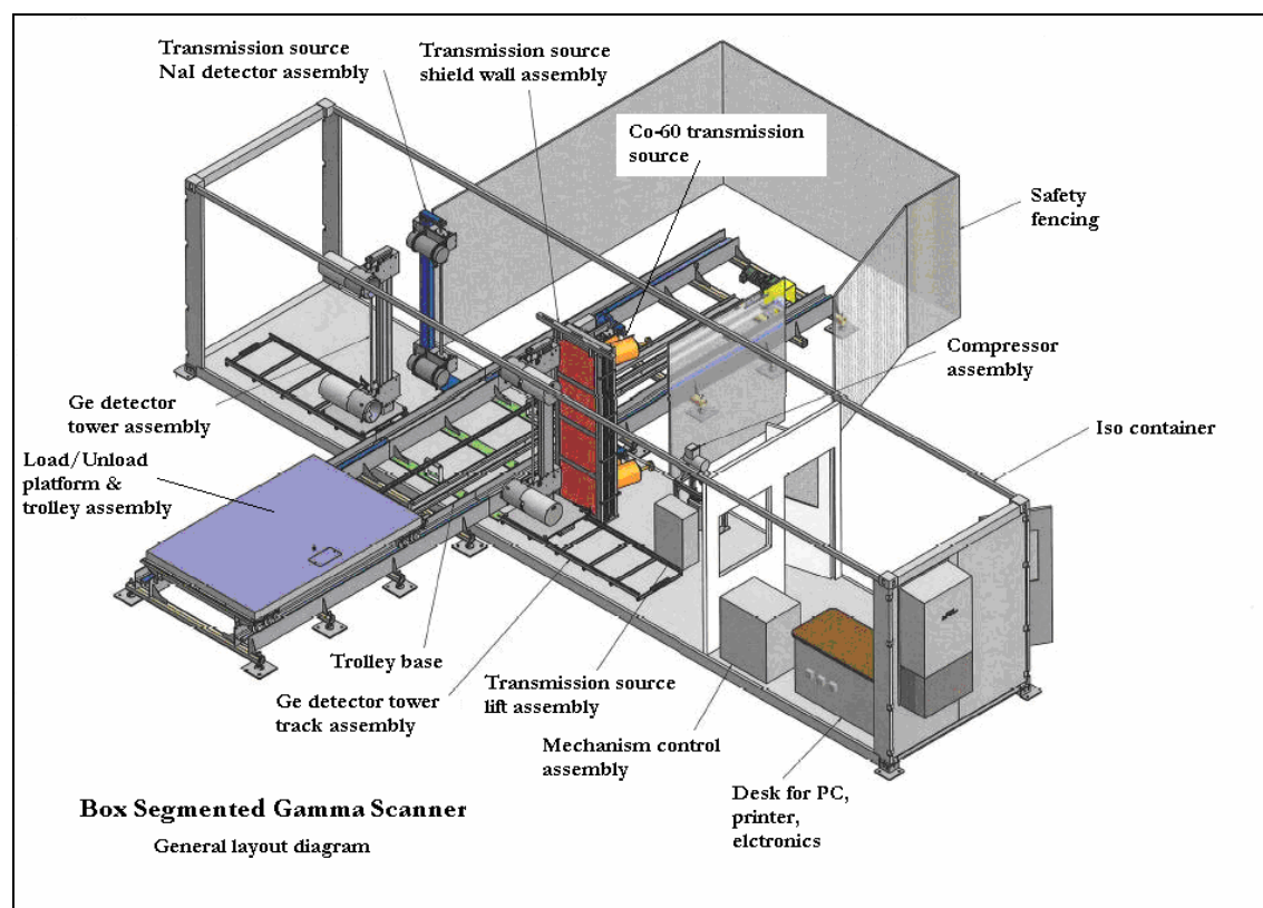
Fig. 1. BSGS general layout.
