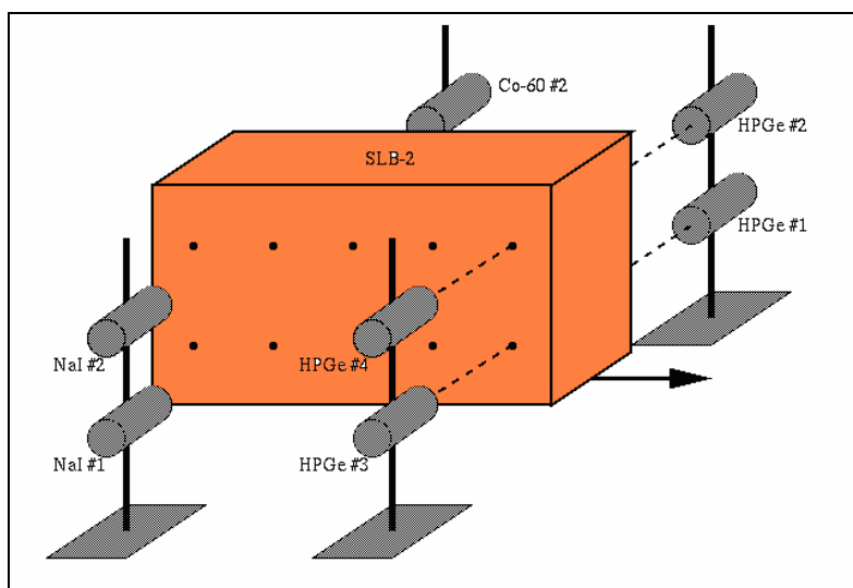
Fig. 3. Schematic of BSGS scanning protocol.
