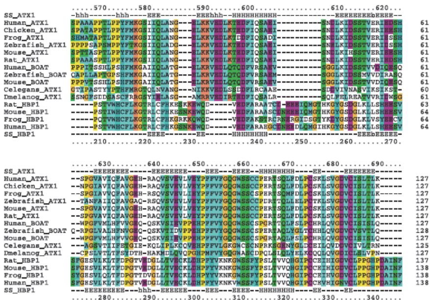
Fig. 7. Alignment based on structural comparison between the AXH from taxin-1 and HBP1 (Chen et al., 2004; de Chiara et al., 2005a). SS_ATX1 and SS_HBP1:experimental secondary structure of ataxin-1 and HBP1.
