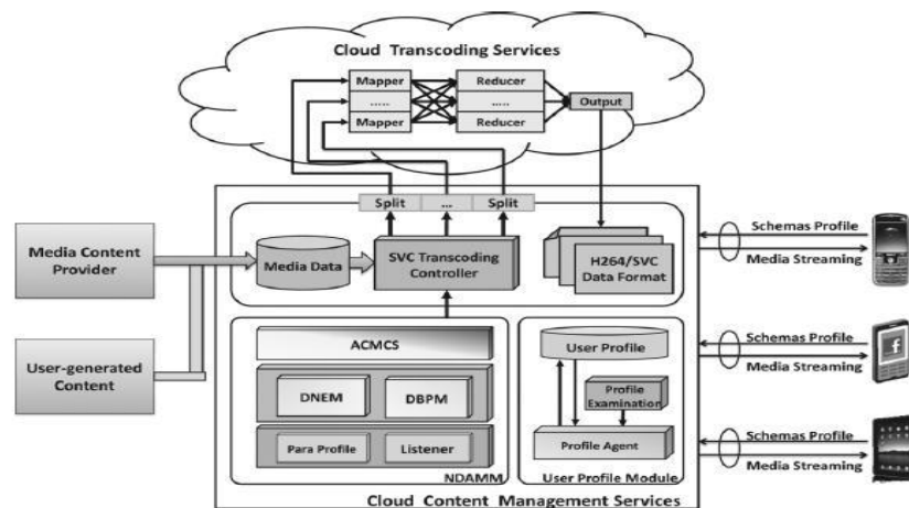
Fig.1: Structure of Cloud-based Mobile Streaming
