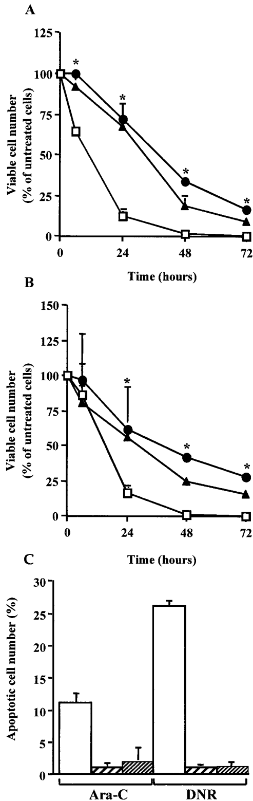
Fig. 2. Effect of PKC \zeta overexpression on drug-induced cytotoxicity. U937-neo (□), U937- \zeta J (●), and U937- \zeta B (▲) cells were incubated or not in the presence of 40 \mu M ara-C (A) or 1 \mu M DNR (B), and cytotoxicity was evaluated after trypan blue exclusion. Results are mean \pm S.E.M. of five independent experiments. *, p < 0.05 for U937- \zeta J and U937- \zeta B cells compared with U937-neo treated cells. C, apoptotic cell number was evaluated at 6 h after DAPI staining in U937-neo (□), U937- \zeta J (▨), and U937- \zeta B (▩) cells treated with 40 \mu M ara-C or 1 \mu M DNR. Results are mean \pm S.E.M. of three independent experiments.
