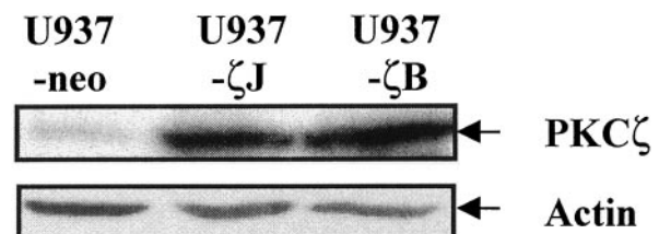
Fig. 1. PKC \zeta expression in PKC \zeta -overexpressing cells. Equal protein concentrations of whole-cell solubilized extracts were prepared from cells transfected with vector (U937-neo) or PKC \zeta (U937- \zeta J and U937- \zeta B). PKC \zeta expression was measured by Western blot analysis as described under Materials and Methods . Results are representative of three independent experiments.
