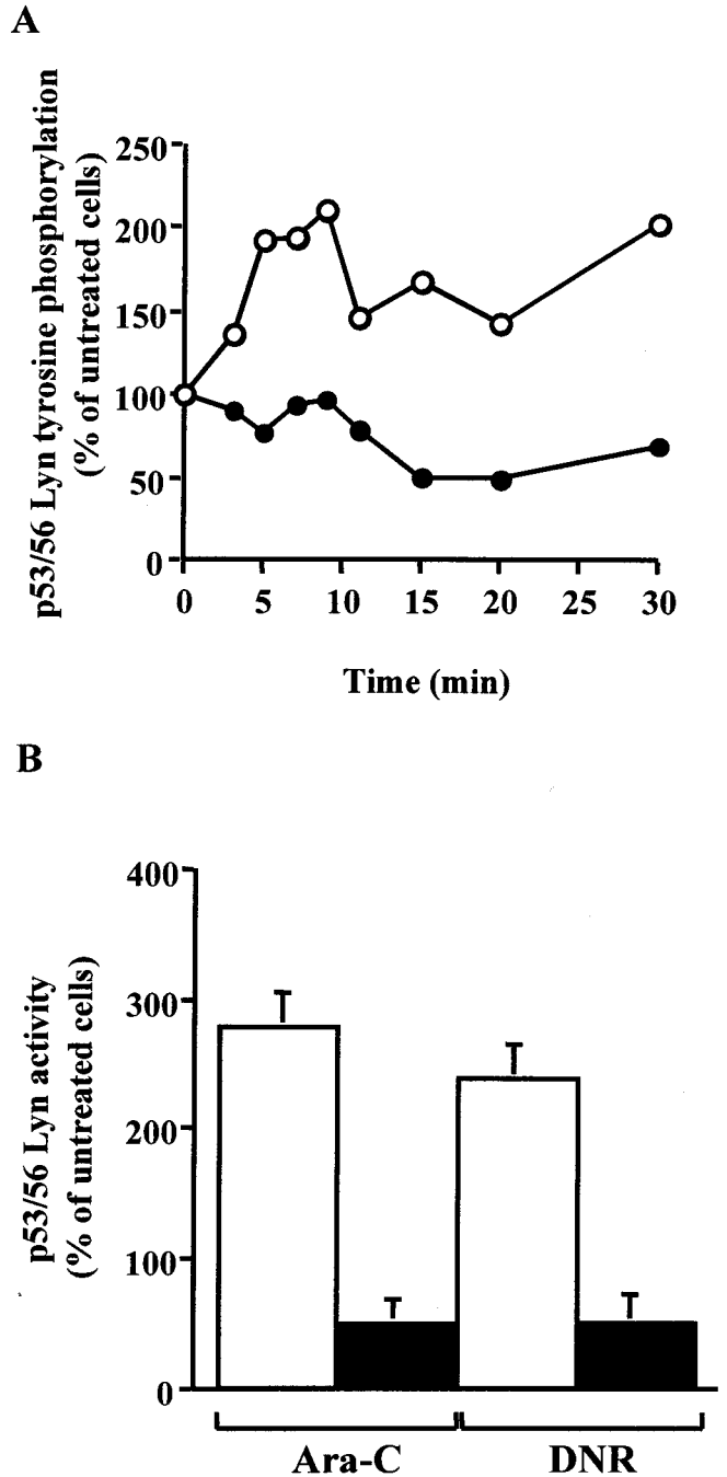
Fig. 7. Effect of PKC \zeta overexpression on drug-induced p53/p56 Lyn activity. A, U937-neo (○) and U937- \zeta J (●) cells were treated with 40 \mu M ara-C, and kinetic of p53/p56 Lyn tyrosine phosphorylation was evaluated after phosphotyrosine immunoprecipitation as described under Materials and Methods . Graph is representative of three experiments. B, U937-neo (□) and U937- \zeta J (■) cells were treated with either 40 \mu M ara-C or 1 \mu M DNR, and p53/p56 Lyn activity was evaluated by an immune kinase assay as described under Materials and Methods . Histograms illustrate p53/p56 Lyn activity at the peak of p53/p56 Lyn kinase stimulation (7–9 min) and are mean \pm S.E.M. of three independent determinations.
