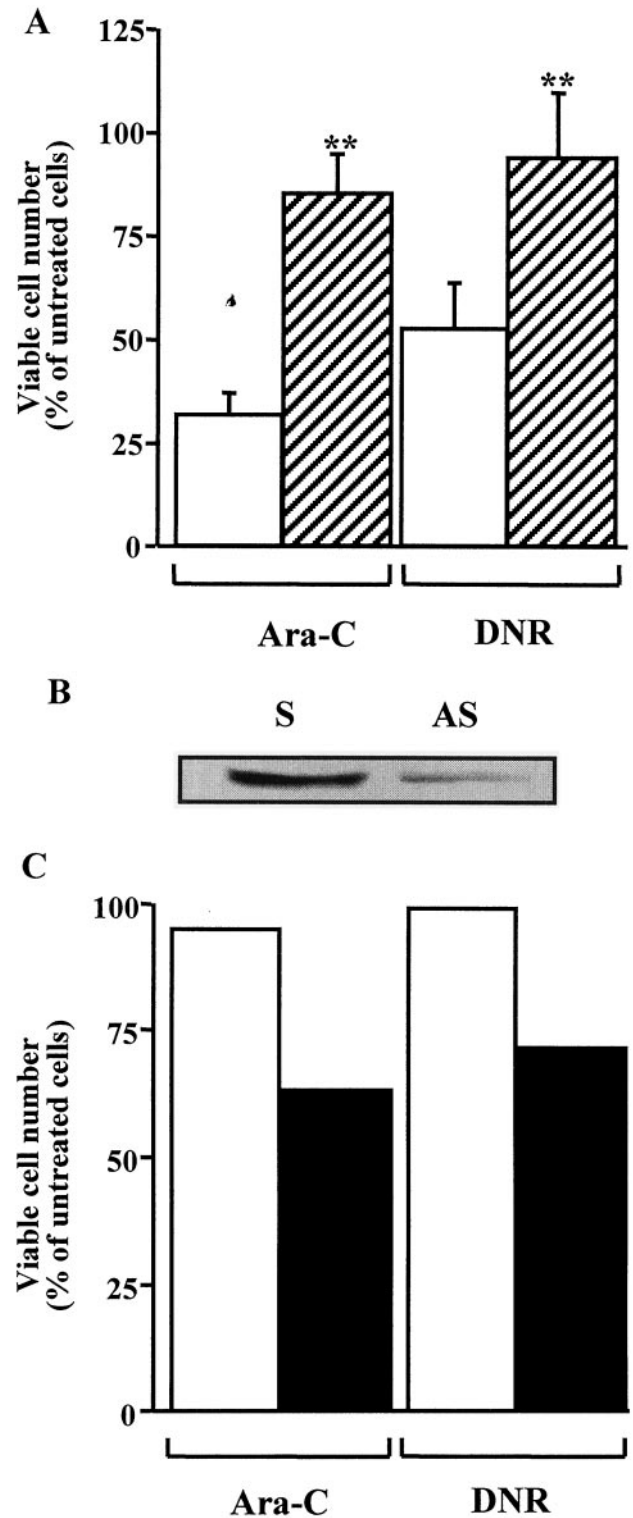
Fig. 3. Effect of antisense oligonucleotides directed against PKC \zeta . A, U937-neo (□) and U937- \zeta J (▨) cells were incubated or not in the presence of 1 \mu M ara-C or 0.1 \mu M DNR for 24 h and cytotoxicity was evaluated after trypan blue exclusion. Results are mean \pm S.E.M. of five independent experiments. **, p < 0.01 compared with U937-neo-treated cells. B, U937- \zeta J cells were preincubated with 10 \mu M antisense (AS, ▩) PKC \zeta or sense (S, □) oligonucleotides for 48 h and then treated with ara-C (1 \mu M) and DNR (0.1 \mu M) for 24 h. PKC \zeta expression was analyzed by Western blot. C, ara-C- and DNR-induced cell cytotoxicity was evaluated at 24 h on oligonucleotide-pretreated U937- \zeta J cells by trypan blue exclusion assay. Results are representative of three independent experiments.
