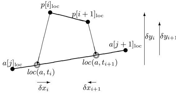
Fig. 6. Definition of \delta x_i , \delta x_{i+1} , \delta y_i and \delta y_{i+1} . Illustrated is the i -th segment of original path p (at top), between points p[i]_{loc} and p[i + 1]_{loc} , and its approximation loc(a, t_i) - loc(a, t_{i+1}) on trajectory a . Observe that this approximation will be part of an a -segment, but that its start and end points may or may not coincide with real data points of a .
