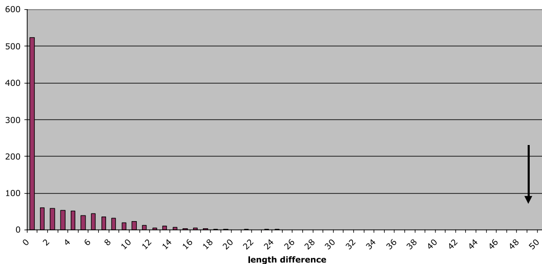
Fig. 3. Parametric bootstrap distribution of tree length differences for all data combined between constrained and optimal topologies constructed from 1000 simulated datasets. Empirical length difference is denoted with the arrow.
