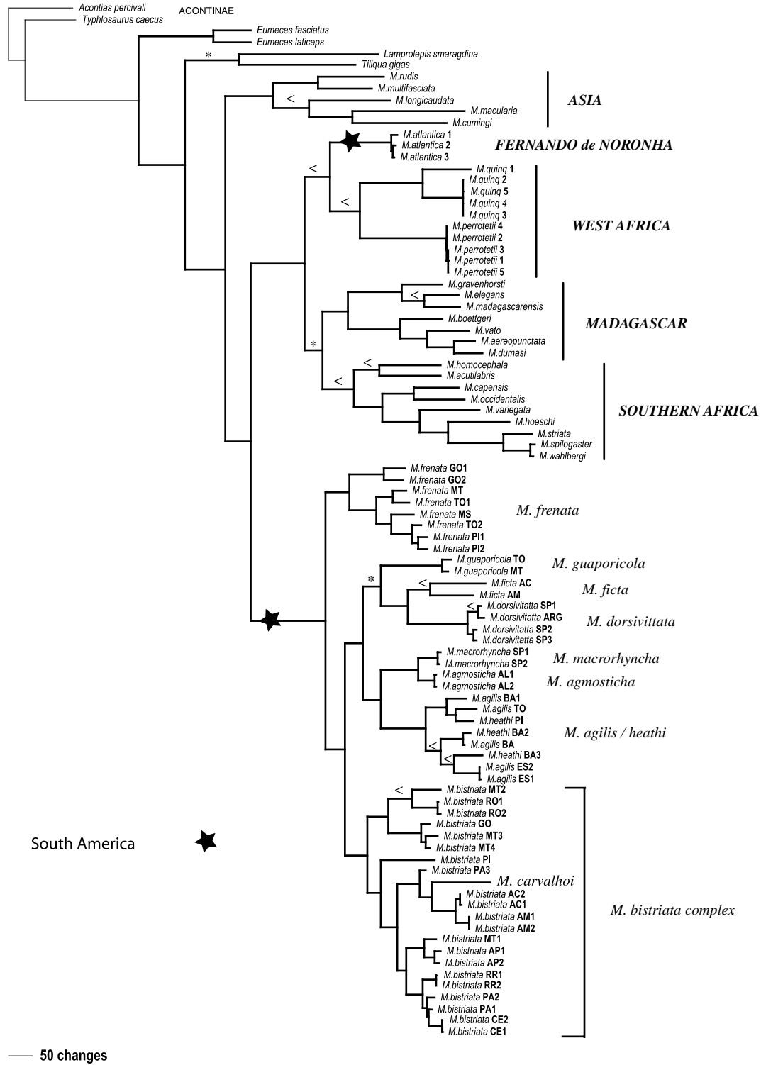
Fig. 2. Partitioned Bayesian analysis of the POY maximum likelihood (POYML) combined data implied alignment, 50% majority rule consensus. Nodes with posterior probabilities below 0.90 are marked <, while 0.90–0.94 are marked *, and all unmarked nodes have values of 0.95–1.0.
