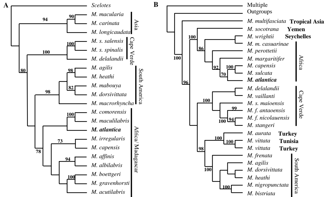
Fig. 1. Topologies from previous molecular studies on Mabuya (redrawn and simplified; branch lengths are not to scale and duplicate species have been removed). (A) Mausfeld et al. (2002) maximum likelihood (ML) topology based on 12S and 16S rRNAs. Numbers above branches are bootstrap proportions based on 100 pseudoreplicates, and values below 50% are not shown. The geographic localities of species are listed to the left. (B) Carranza and Arnold (2003) ML topology (greatly simplified with duplicate taxa removed), based on cyt b , 12S and 16S rRNAs. Numbers on the tree are Bayesian posterior probabilities, with values below 50 not shown.
