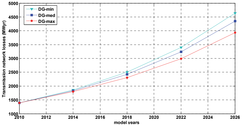
Fig. 3. Transmission network losses
