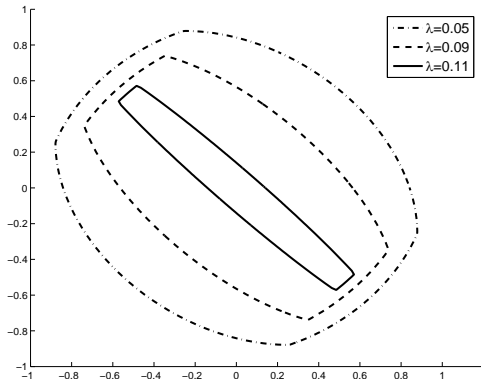
Fig. 2. Unit balls of \|\cdot\|_{G_\lambda} for the SLS (6).
