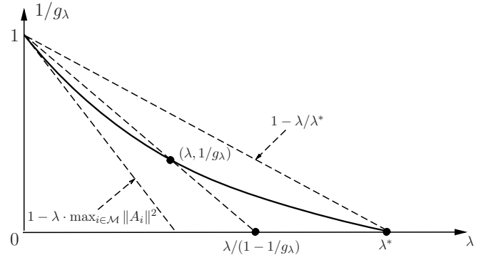
Fig. 1. Plot of the function 1/g_\lambda (in solid line).
