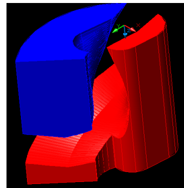
Figure 6: Inflector with the “bended” electrodes.
