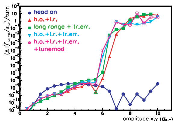
Figure 1: Change of action variance per turn vs. start amplitude x_{\text{start}} (= y_{\text{start}}) in units of rms beam size for two IPs [2].
