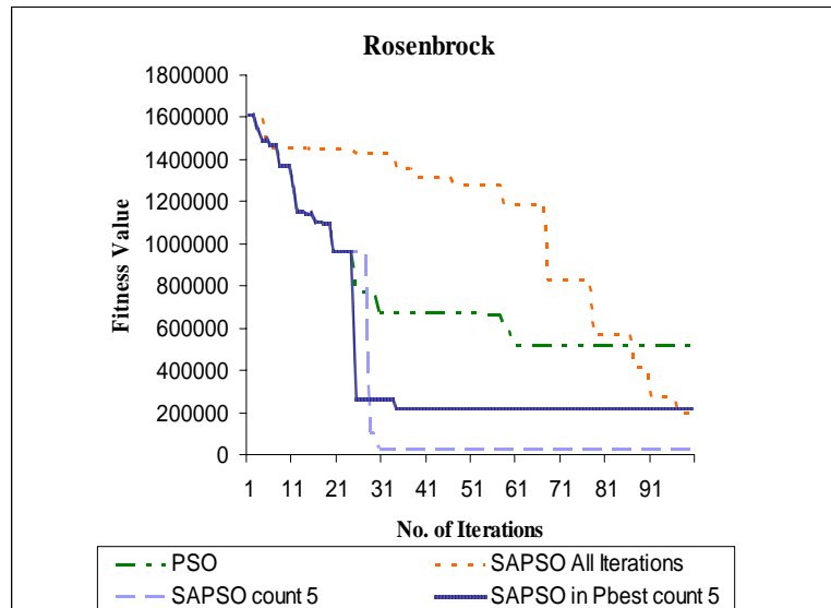
Fig. 6. Fitness value obtained from Rosenbrock function
