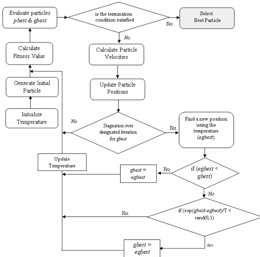
Fig. 2. SAPSO when gbest particle stagnates
