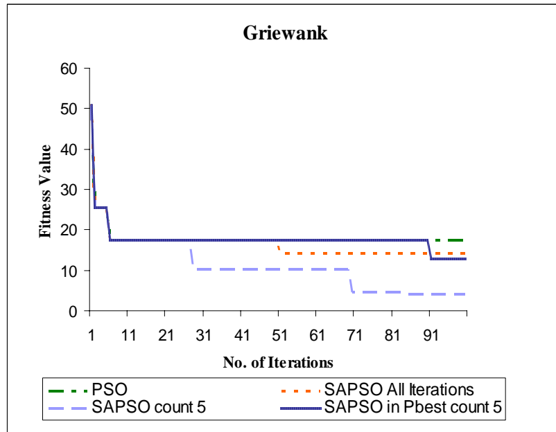
Fig. 5. Fitness value obtained from Griewank function
