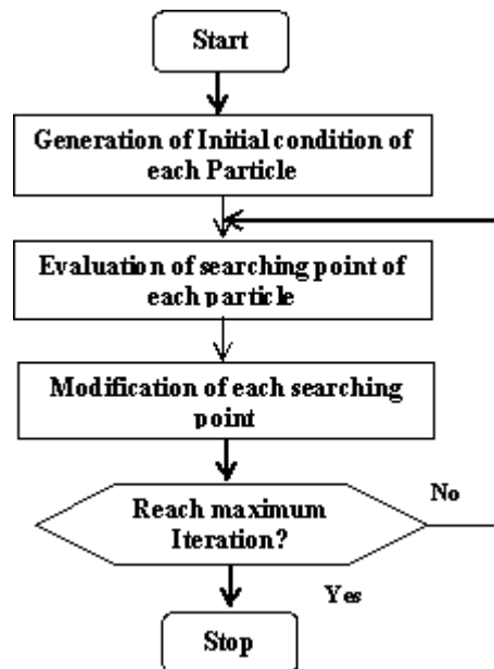
Fig. 1. Standard PSO
