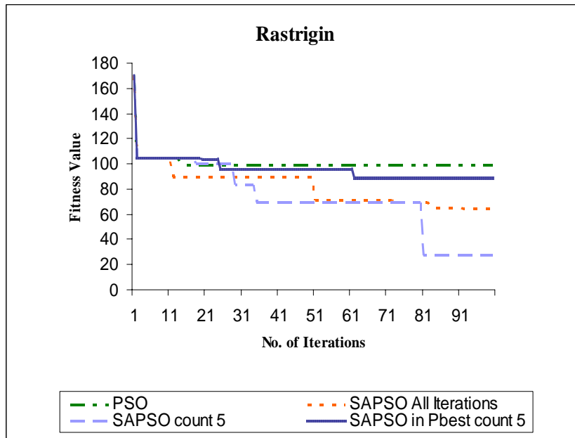
Fig. 4. Fitness value obtained from Rastrigin function
