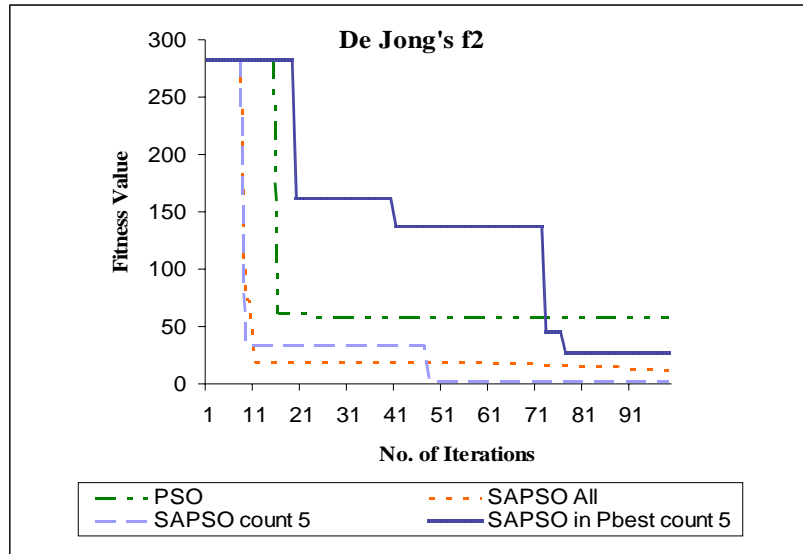
Fig. 3. Fitness value obtained from De Jong's function
