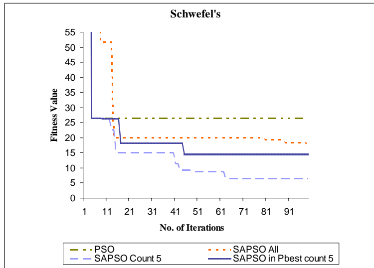
Fig.7. Fitness value obtained from Schwefel function
