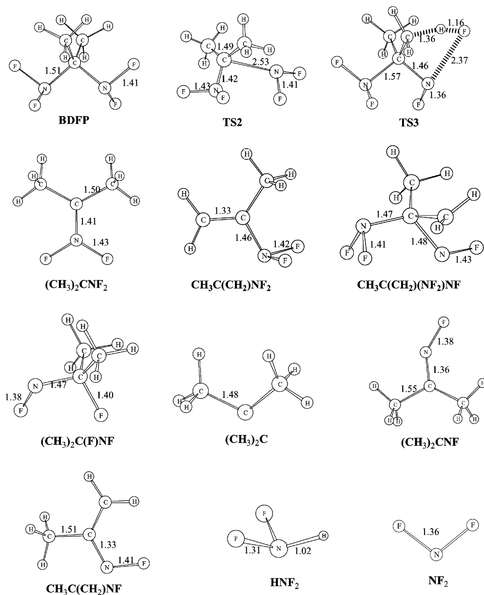
Fig. 5. B3LYP/6-31G(d,p) optimized geometries for the species involved in the decomposition of BDFP and (CH 3 ) 2 CNF 2 . For simplicity only important parameters are labeled.
