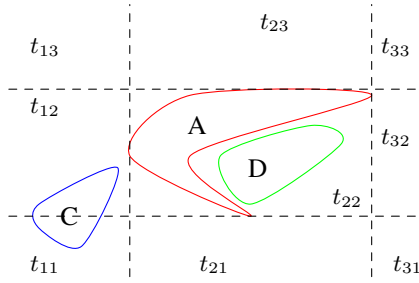
Figure 4: The MBR of object A and the tiling of the plane
