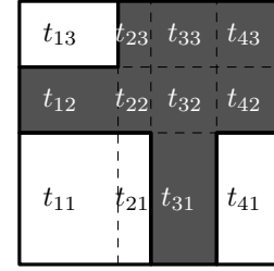
Figure 7: A unit that requires representation in the 5th granularity level
