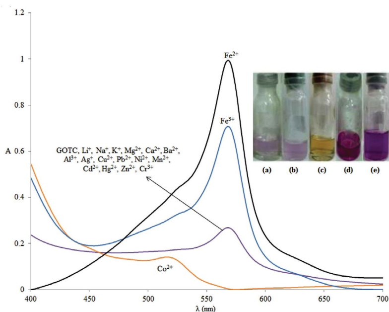
Fig. 3. The color changes of GOTC upon addition of various metal ions: (a) free GOTC ( 0.2 \text{ mg ml}^{-1} ), (b) after addition of relevant metal ions ( \text{Li}^+ , \text{Na}^+ , \text{K}^+ , \text{Mg}^{2+} , \text{Ca}^{2+} , \text{Ba}^{2+} , \text{Al}^{3+} , \text{Ag}^+ , \text{Cu}^{2+} , \text{Pb}^{2+} , \text{Ni}^{2+} , \text{Mn}^{2+} , \text{Cd}^{2+} , \text{Hg}^{2+} , \text{Zn}^{2+} and \text{Cr}^{3+} ), (c) \text{Co}^{2+} , (d) \text{Fe}^{3+} and (e) \text{Fe}^{2+} .
