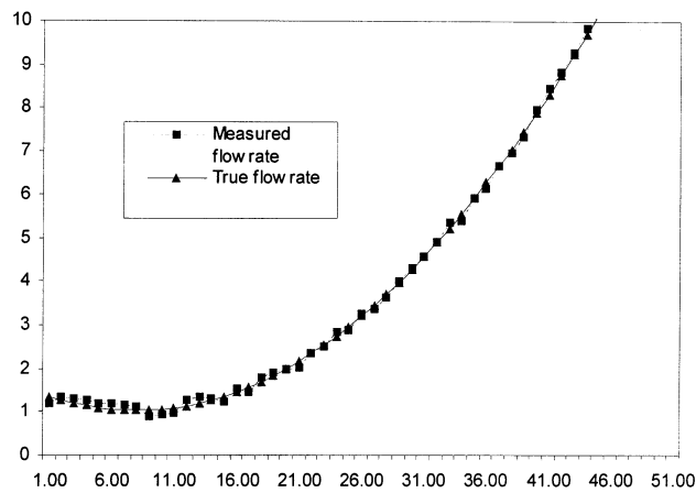
Fig. 4. Measurements and true values of f_2 .
