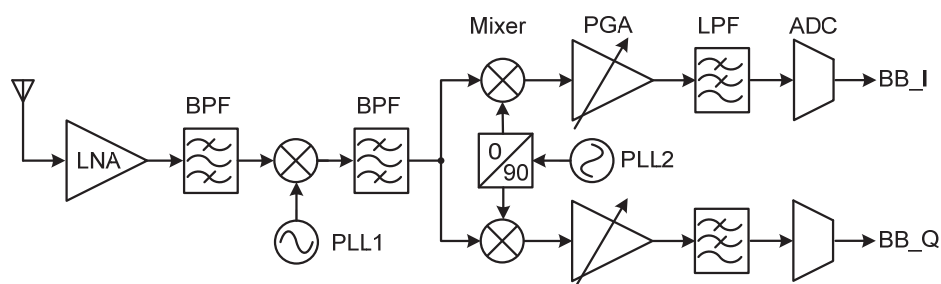
Fig. 1. Superheterodyne Receiver
