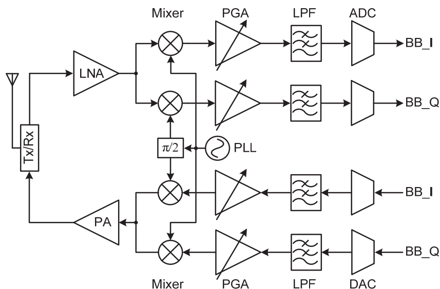
Fig. 2. Direct-conversion Transceiver
