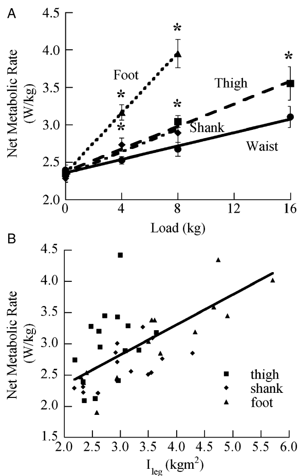
FIGURE 2— A, Mean net metabolic rate ( W \cdot kg^{-1} ) vs load mass ( m ) and location. B, Net metabolic rate vs moment of inertia of the leg ( I_{leg} ) for each subject. The increase in net metabolic rate was greatest with foot loads, similar for thigh and shank loads, and least for waist loads. Linear regression equations for panel A: Waist watts per kilogram = 2.36 + 0.045m , r^2 = 0.65 . Thigh watts per kilogram = 2.38 + 0.075m , r^2 = 0.72 . Shank watts per kilogram = 2.34 + 0.076m , r^2 = 0.61 . Foot watts per kilogram = 2.36 + 0.20m , r^2 = 0.85 . Linear regression equations for panel B: watts per kilogram = 1.3774 + 0.4831I_{leg} , r^2 = 0.43 . * Significant difference, load location vs waist load.
