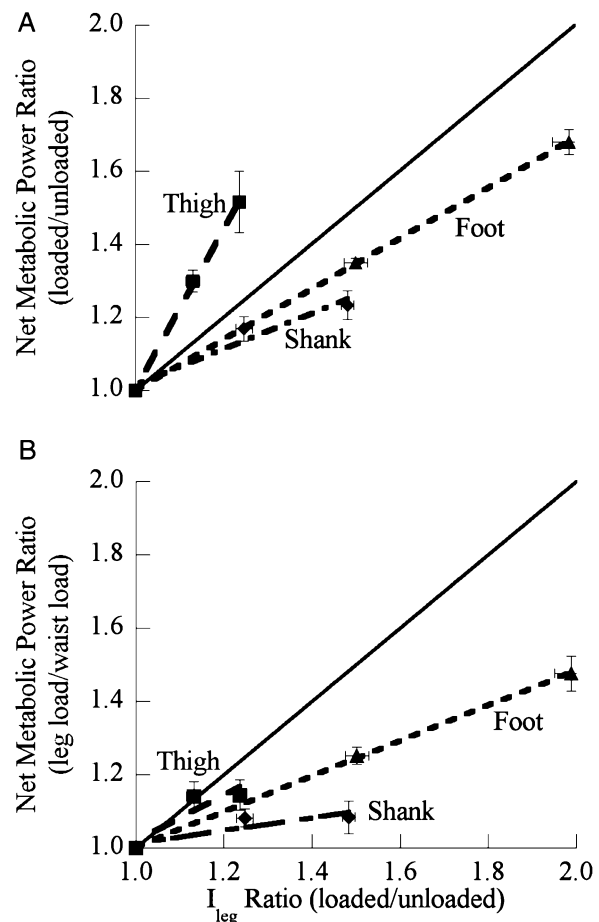
FIGURE 7—A, Net metabolic power ratio (load/no load) vs I_{\text{leg}} ratio (load/no load). The thin solid line is the line of identity. Relative increases in I_{\text{leg}} with thigh loading resulted in greater increases in net metabolic rate than more distal loading locations. Linear regression equations for panel A: thigh metabolic ratio = -0.74 + 1.81I_{\text{ratio}} , r^2 = 0.50 . Shank metabolic ratio = 0.63749 + 0.40916I_{\text{ratio}} , r^2 = 0.46 . Foot metabolic ratio = 0.32639 + 0.68067I_{\text{ratio}} , r^2 = 0.98 . B, Metabolic rate ratio (load/waist load) vs I_{\text{leg}} ratio (load/waist load). Expressed relative to waist loads, increases in I_{\text{leg}} resulted in similar increases in net metabolic rate with thigh and foot loading.
