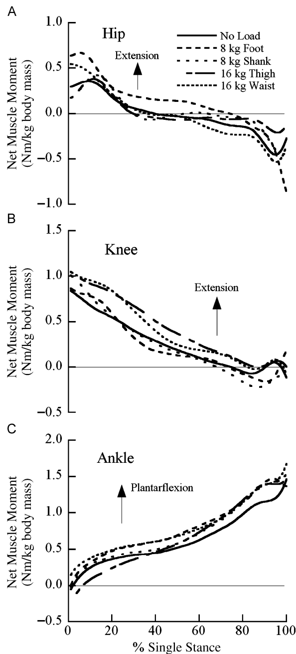
FIGURE 4 —Net muscle moments per kilogram of body mass vs percent single stance for the hip (A), knee (B), and ankle (C) for the no-load and maximum segment load conditions. Stride begins at heel strike (i.e., 0% stride = heel strike). Values are means for all subjects. Positive moments are extensor. Net muscle-moment patterns during single stance were similar across loading conditions. Peak hip extensor and flexor moments during early and late single stance, respectively, were significantly greater with the 8-kg foot vs no-load trials. Peak knee and ankle net muscle moments were not significantly different across loading conditions.
