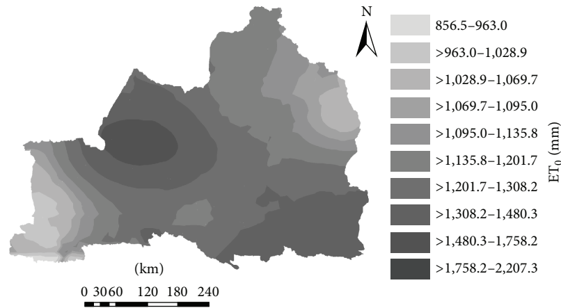
FIGURE 6: Spatial distribution of average monthly ET_0 from April to October of 1962–2010 in Northern Xinjiang.
