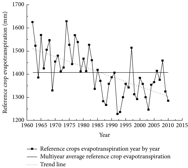
FIGURE 2: Annual variation of average ET_0 in Northern Xinjiang.
