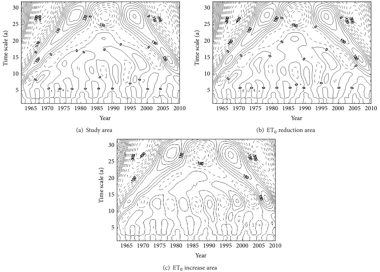
FIGURE 4: Morlet wavelet transform of average ET_0 .
