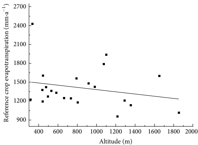
FIGURE 7: Tendency of ET_0 with altitude.
