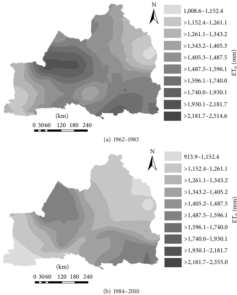
FIGURE 5: Spatial distribution of average annual ET_0 between 1962 and 1983 and 1984 and 2010 in Northern Xinjiang.
