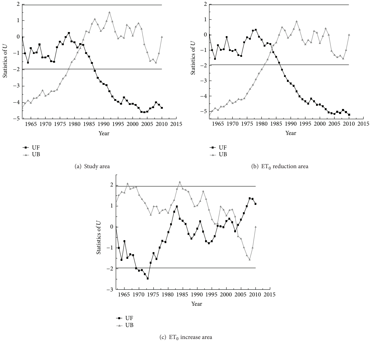
FIGURE 3: Mann-Kendall test of average ET 0 .
