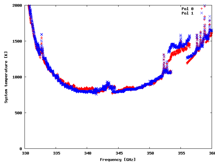
Figure 3. Example of system noise temperature "jump" around 355 GHz.
