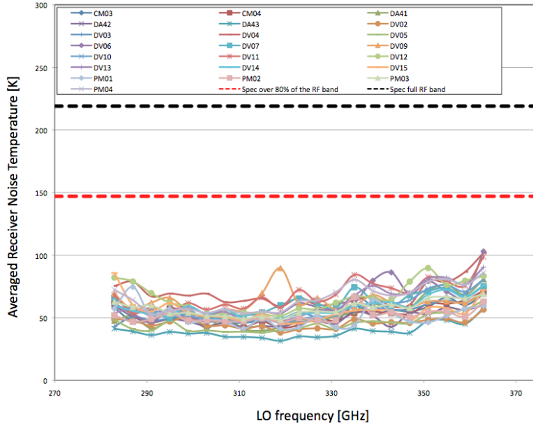
Figure 6. Receiver noise temperature with 4.0–8.0 GHz IF as a function of LO frequency. Four IF outputs corresponding to both polarizations and sidebands (USB/LSB) receiver noise are averaged
