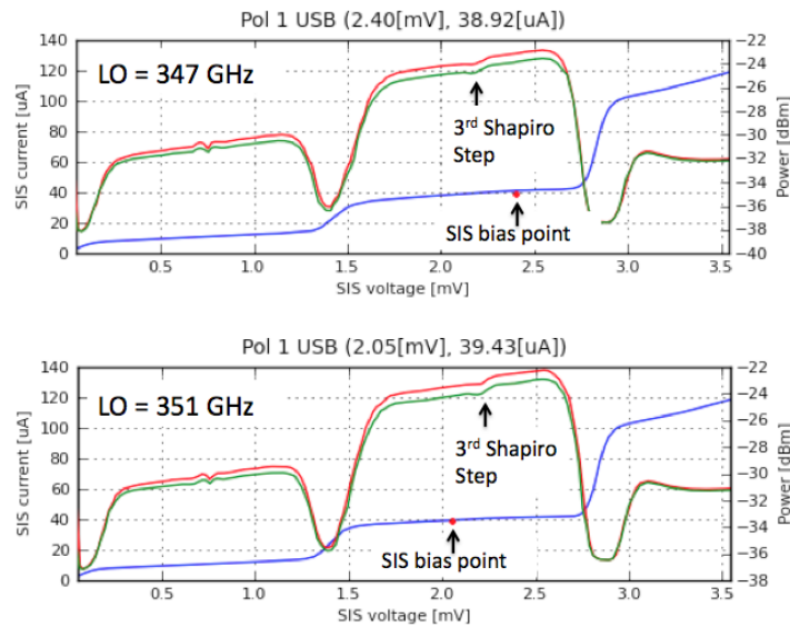
Figure 2. Measured Pumped SIS I-V curves (blue) and two IF-output-powers corresponding to Hot load (~80 C: red) and Ambient load (~15 C: green) signal inputs. Top: LO frequency @ 347 GHz. Bottom: LO frequency is 351 GHz.
