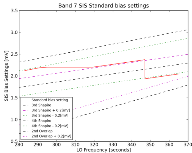
Figure 5. Band 7 Standard SIS bias setting curve that has been implemented. The figure also shows the avoided regions near the third and fourth Shapiro steps and the photon step overlap.
