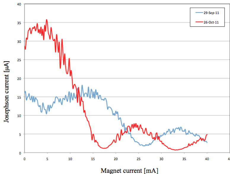
Figure 1. Example of worst case of Band 7 magnetic field scans on different days on antenna. Note that these data were taken before implementing de-flux/de- magnetize procedure.
