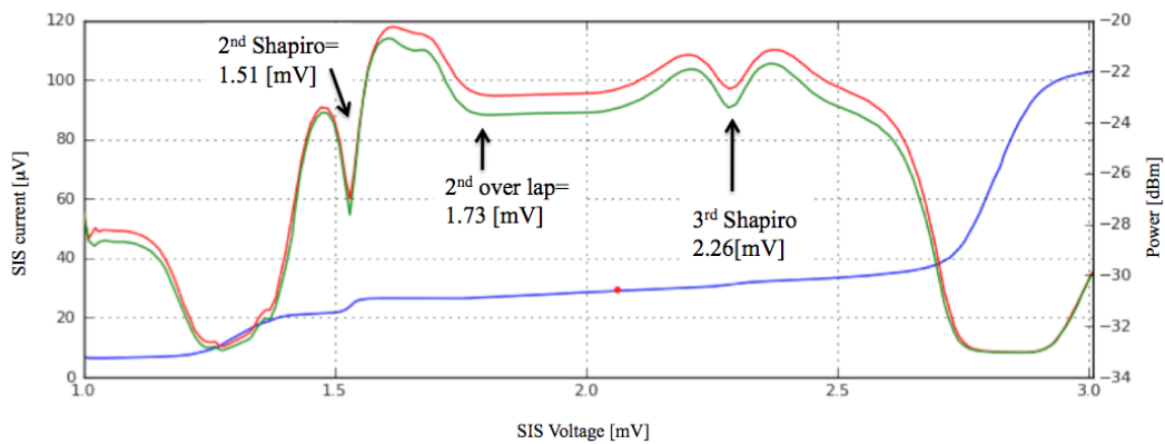
Figure 4. Measured Pumped SIS IV curves (blue) and IF output powers corresponding to Hot (~80 C: red) and Ambient (~15 C: green) loads inputs @ LO = 365 GHz. Note the plot was taken in ‘un-optimized’ mixer tuning to see Shapiro steps and photon step overlap effects.
