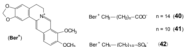
Fig. 13. Chemical structure of the berberine derivatives 40-42
