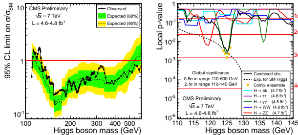
Figure 1: Exclusion confidence level for the combined SM Higgs search in the full mass range 110–600 GeV (left) and combined local p-value for the SM Higgs search (right).
