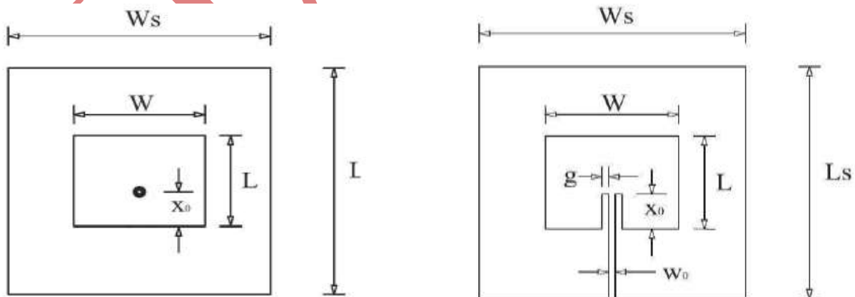
Fig.1 Geometrical Detail of Probe Fed Patch Antenna Fig. 2 Geometrical Detail of Inset Fed Micro Stripline Fed Patch Antenna.
