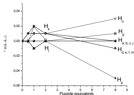
Figure 5. 1 H NMR shifts for the protons of receptor 3d in the presence of increasing quantities of fluoride anion (DMSO-d 6 ).
