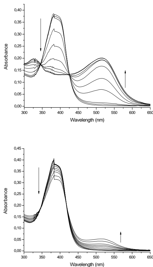
Figure 2. UV-Vis titration of receptors 3c ( 1.2 \times 10^{-5} mol dm -3 ) with fluoride (top) and acetate (bottom) anions (0-30 equiv) in acetonitrile.
