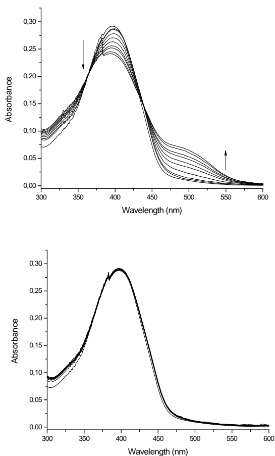
Figure 3. UV-Vis titration of receptors 3d ( 1.2 \times 10^{-5} mol dm -3 ) with fluoride (top) and acetate (bottom) anions (0-30 equiv) in acetonitrile.
