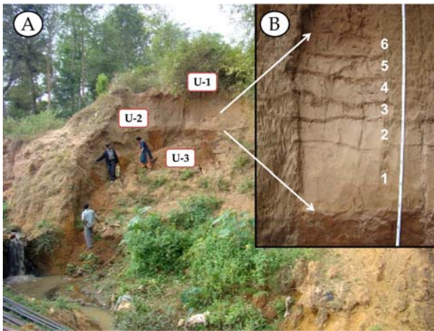
Fig. 2. (A). Photograph showing the general view of the alluvial deposits exposed on the left bank of the Kaveri River at Siddapur. (B) Enlarged view of the six flood couplets (1-6) seen in the middle unit (U-2) in A.
