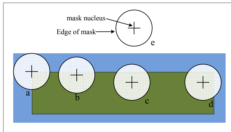
Fig. 1 USAN(Univalued Segment Assimilating Nucleus)
