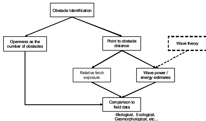
Figure 1. Flow diagram illustrating key steps in cartographic fetch modeling. All models include some method for obstacle identification, but vary in which additional steps they include and how they are achieved.
