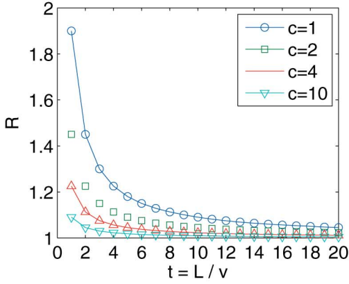
Fig. 5. Approximation ratio as the parameters change.
