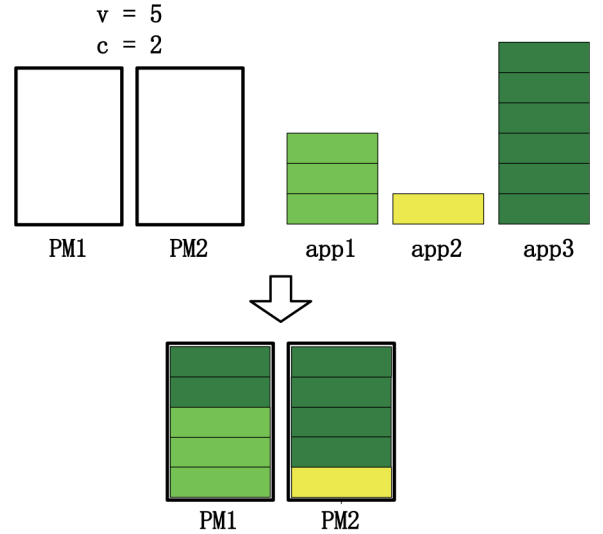
Fig. 3. Class constrained bin packing (CCBP).
