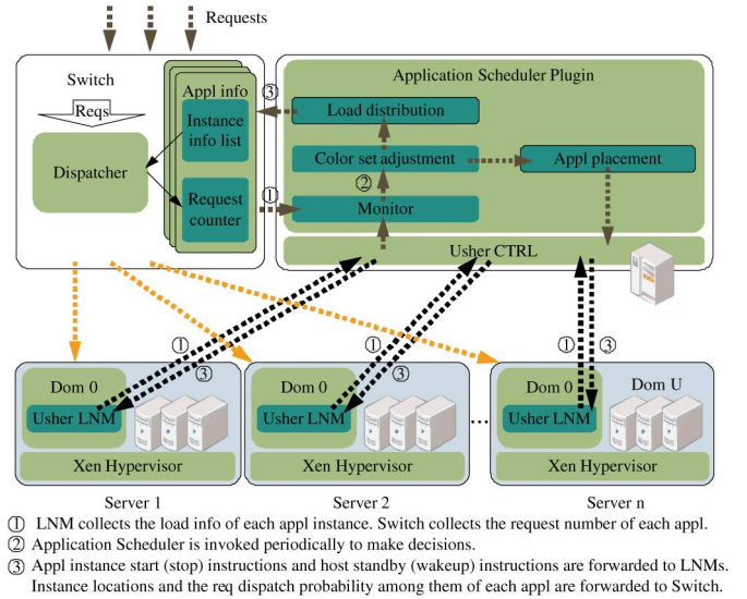
Fig. 2. Overview of the system architecture.
