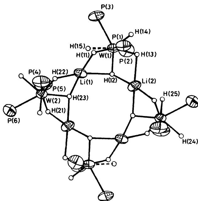
Figure 2. The structure of \{[(\text{Me}_3\text{P})_3\text{WH}_5]\text{Li}\}_4 ( E ). The methyl groups have been omitted for clarity and one terminal hydrogen on W(1) (shown bonded via a dashed line) was not identified experimentally
