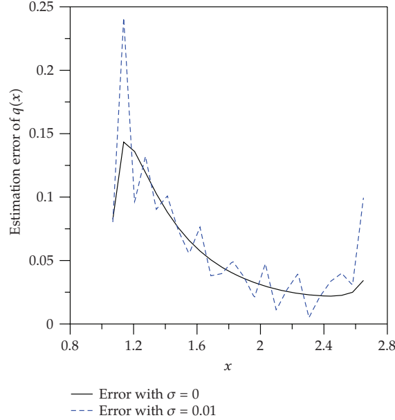
Figure 2: Example 6.2 of identifying q(x) , the estimation errors were plotted.
