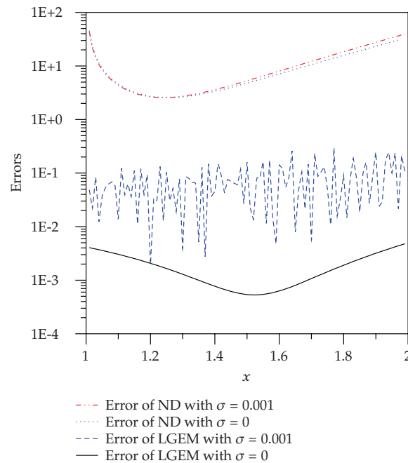
Figure 6: Example 6.6 comparing the estimation errors of p(x) under random disturbances with \sigma = 0 and \sigma = 0.001 .
