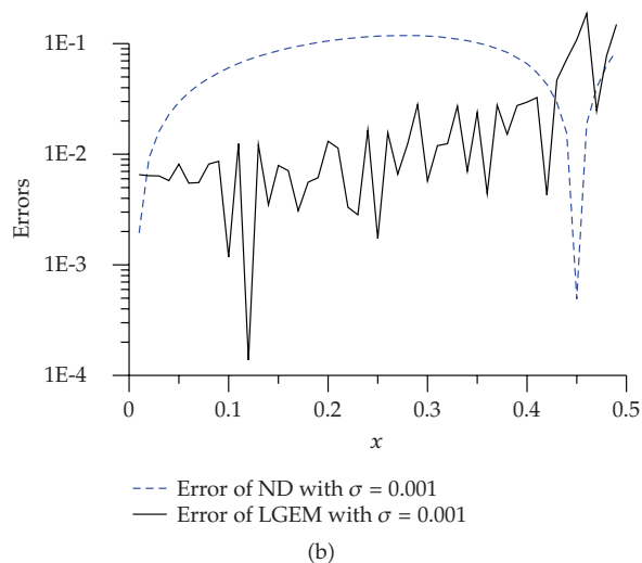
Figure 5: Example 6.5 comparing the estimation errors of p(x) : (a) definite disturbances with \delta = 0, 0.02 , and (b) random disturbance with \sigma = 0.001 .
