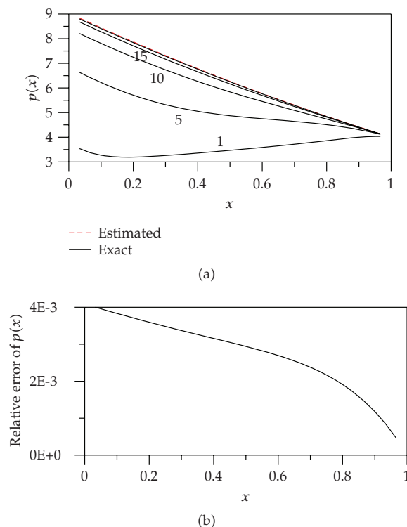
Figure 3: Example 6.3 by using an iterative method: (a) comparing estimated and exact p(x) , and (b) plotting the relative error of estimation.
