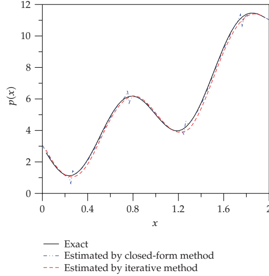
Figure 4: In Example 6.4 we compare exact p(x) with the estimated ones by using an iterative method and a closed-form method.
