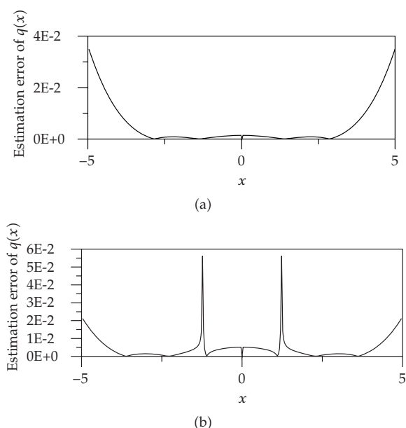
Figure 1: Example 6.1 of identifying the Schrödinger equation (a) plotting the estimation error by using the second spectral function, while (b) by using the fourth spectral function.
