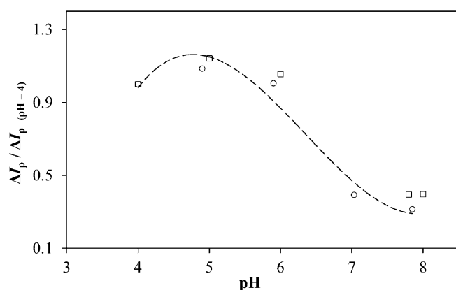
Fig. 7. Comparison of theoretical ( \square ) and experimental ( \circ ) net peak currents for alizarin as a function of pH. Simulations have been performed for a simple surface confined electrode reactions assuming electron transfer coefficient \alpha=0.5 , n=2 , and apparent standard rate constant values listed in Table 1. For consistent comparison, both theoretical and experimental net peak currents ( \Delta I_p ) are normalized with respect to the one corresponding to the lowest pH value ( \Delta I_{p(\text{pH}4)} ).
