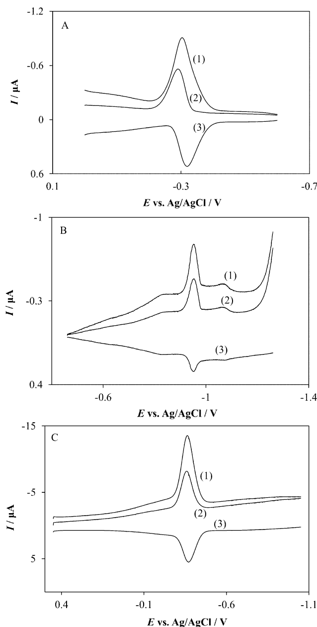
Fig. 1. Typical SW voltammograms recorded in a BR buffer following an adsorptive accumulation of: (A) 2 \mu mol/L alizarin at pH 9 at HMDE ( t_{acc} = 30 s, E_{acc} = 0.0 V); (B) 5 \mu mol/L vitamin B12 at pH 4 at HMDE ( t_{acc} = 90 s, E_{acc} = -0.4 V); and (C) 2 \mu mol/L vitamin K2 at pH 9 at GCE ( t_{acc} = 30 s, E_{acc} = 0.5 V). The parameters of the potential modulation are: f = 25 Hz, E_{sw} = 50 mV and \Delta E = 1 mV. Numbers 1, 2, and 3 on the plots refer to the net, forward (cathodic) and backward (anodic) components of the SW voltammetric response.
