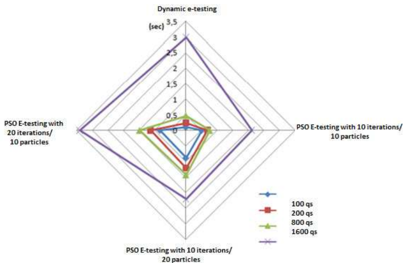
Fig. 13. Average Execution Times for the Selection of One Question, in Various Forms of e-assessment, using Item Banks of Variable Dimensions
