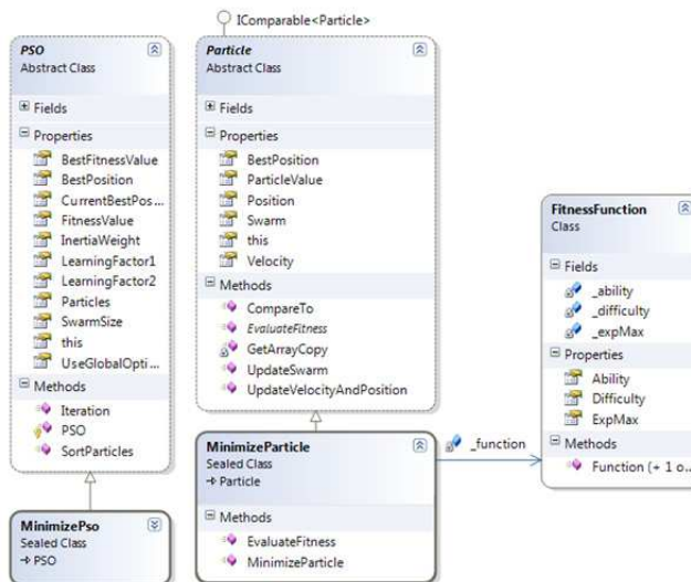
Fig. 9. The Class Diagram of the PSO Algorithm
