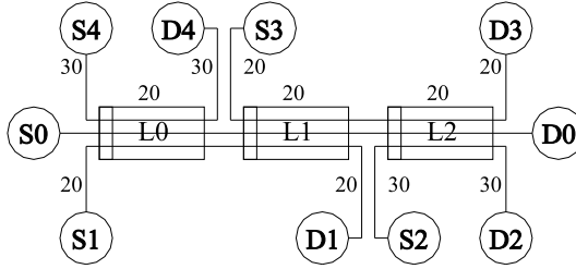
Fig. 2. Network Simulated.
