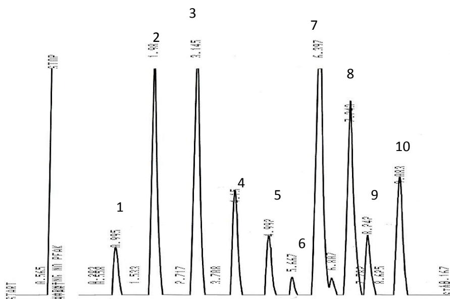
Figure 4- HPLC profile of Convolvulus arvensis Phenols (1) Caffeic acid, (2) Thujone, (3) Cymene, (4) Ferulic acid, (5) Isoferulic acid, (6) Cimircoside, (7) \beta -pellandrene, (8) Gentisic acid, (9) Leutoline, (10) Coumaric acid .
