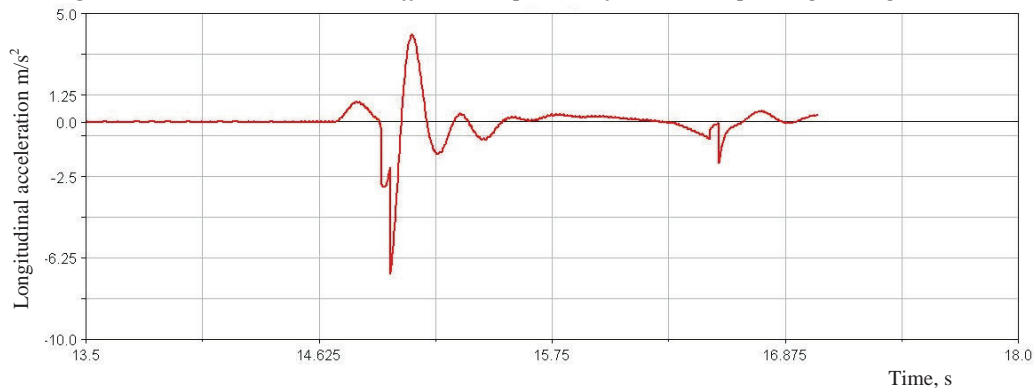
Fig. 8. Time graph of longitudinal acceleration effects on operator while crossing a pothole at the velocity of 2 m/s, for maximum lift height of loader's bucket
