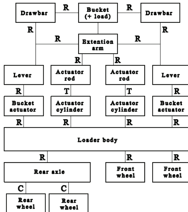
Fig.1. Diagram showing types of connections between particular elements in the numerical model of the Ł34 loader: R-rotating joint, T-travelling joint, C-cylindrical joint
