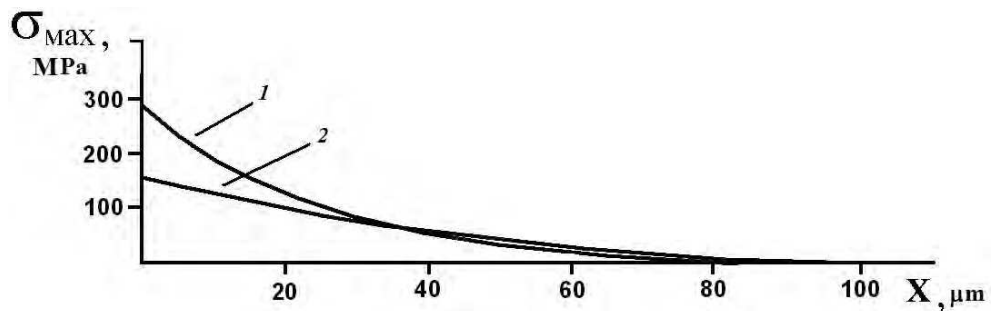
Fig. 34. Distribution of stresses in a single column by length 100\ \mu\text{m} , the column of the different cross-section sizes: 1 - d_1 = 0,5\ \mu\text{m} , d_2 = 1,0\ \mu\text{m} ; 2 - d_1 = 0,5\ \mu\text{m} , d_2 = 0,5\ \mu\text{m}
