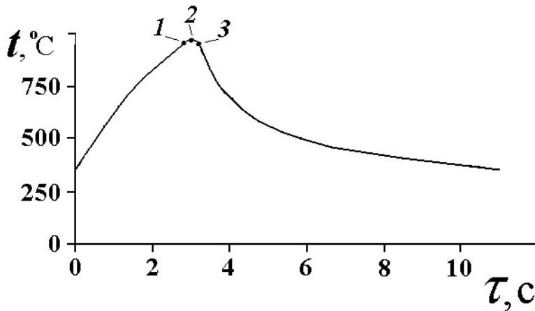
Fig. 17. Heating thermogram.
