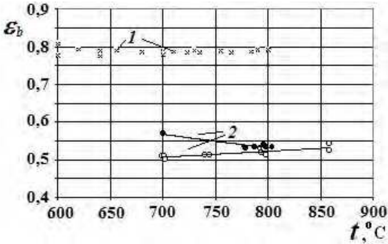
Fig. 14. Blackness degree \epsilon_b depending on temperature
