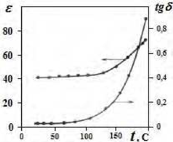
Fig. 9. Parameters \varepsilon and tg\delta depending on temperature
