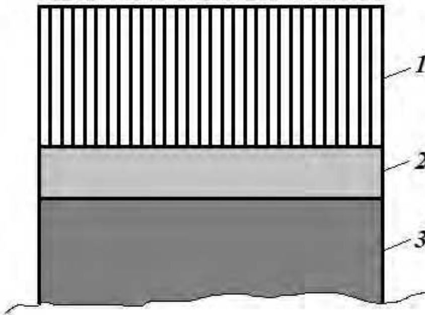
Fig. 3. Thermal barrier coating system: 1 - ceramic coating ZrO_2-8\%Y_2O_3 , 2 - bond coating MCrAlY , 3 - superalloy
