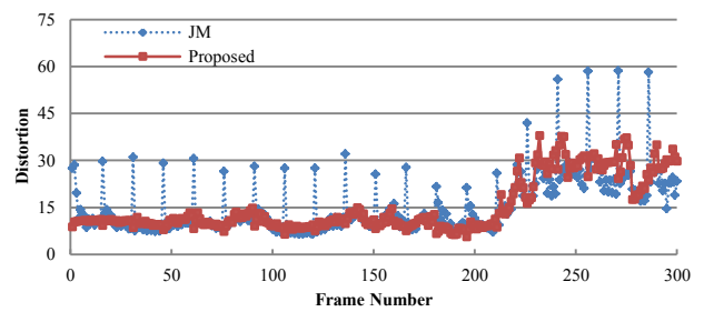
Fig. 2 Frame level distortion between JM and proposed RC in Foreman sequence at 500kbps.
