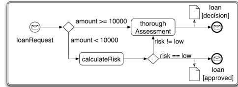
Fig. 3. The Bank Loan BPEL Process [35]
