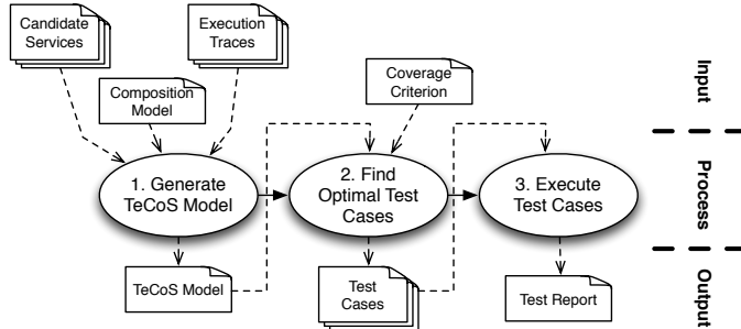
Fig. 4. Simplified TeCoS Approach
