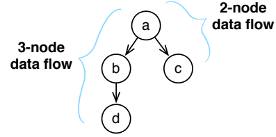
Fig. 5. Example K-Node Data Flows
