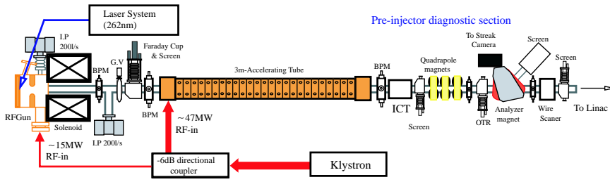
Figure 1: Layout of ATF pre-injector. RF power from a klystron is distributed to the RF gun and the accelerating structure. Many instrumentation devices are implemented. In actual system, the cathode load-lock system is connected directly to the gun cavity.
