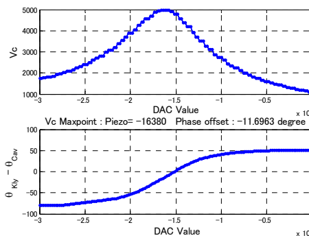
Figure 6: Resonance search by scanning DAC-offset. Phase is calibrated by setting \Delta\theta=0 at the maximum point of V_c .
