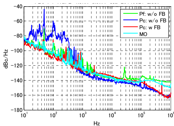
Figure 10: Results of phase noise measurements of MLSC2 using a signal source analyzer; green and blue: input RF and cavity signal w/o feedback, red: cavity signal with feedback, cyan: MO.
