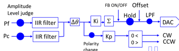
Figure 5: Schematic diagram of tuner control.
